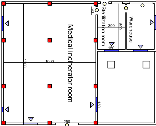
Ground floor B2 scale 1/100
