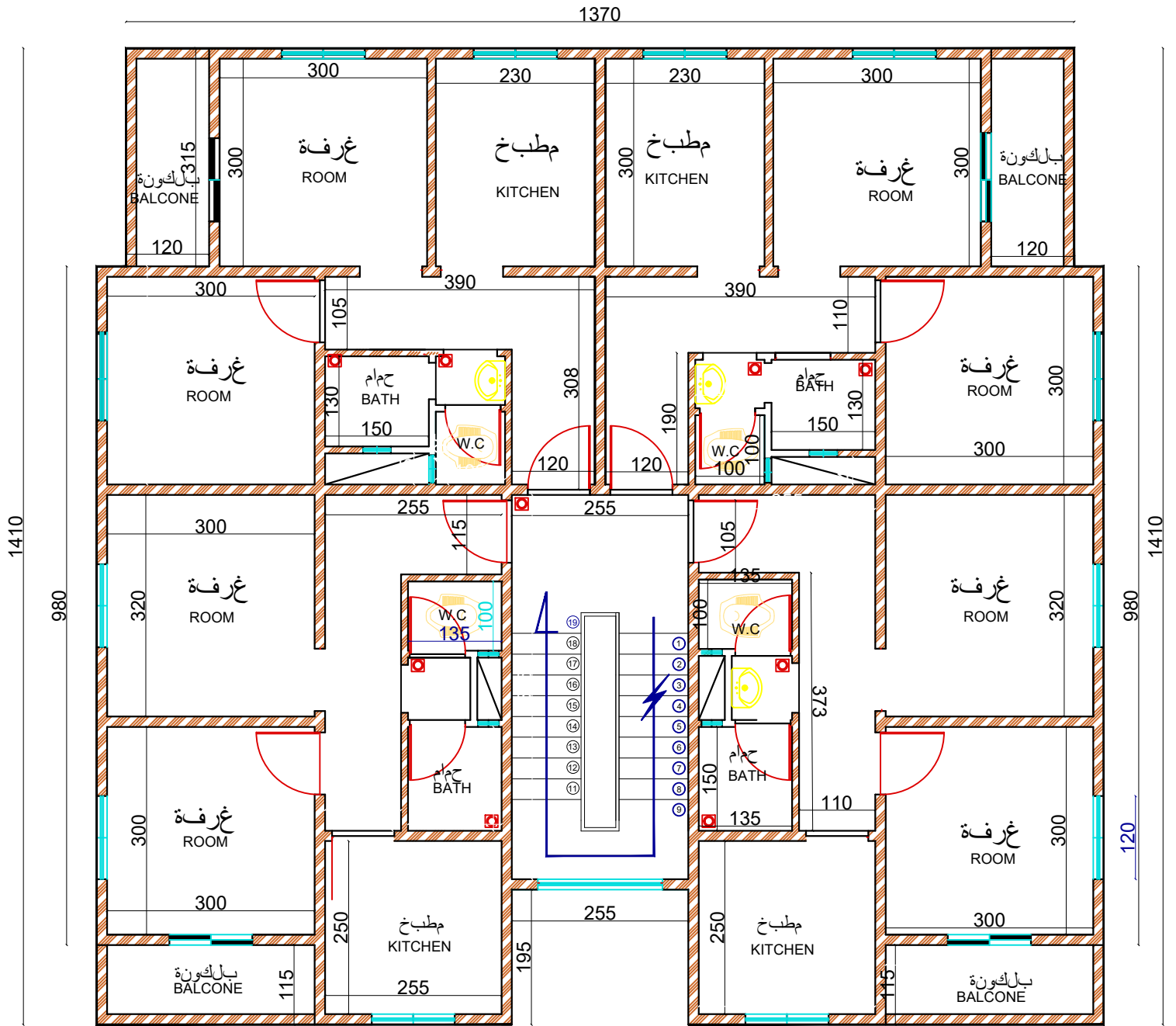
FIRST FLOOR
